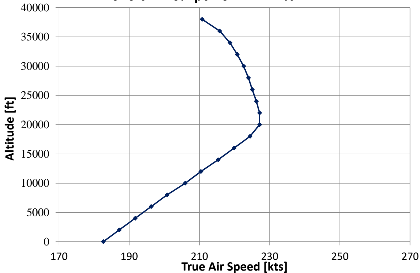
CRUISE - 75% power - 1141 lbs
